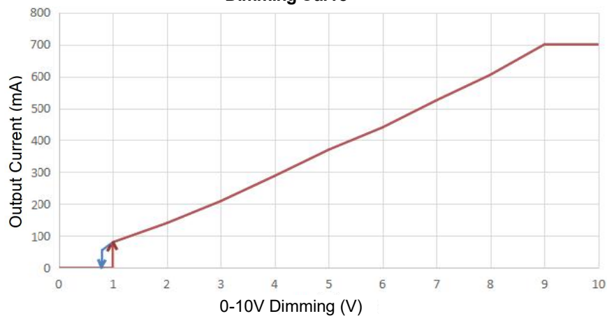
Dimming Curve
