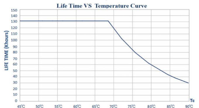
Lifespan
